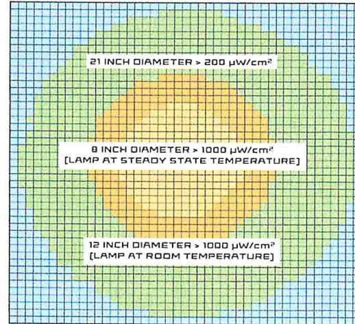
BEAM PROFILE AT 15 INCHES
