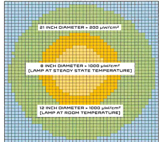
BEAM PROFILE AT 15 INCHES
